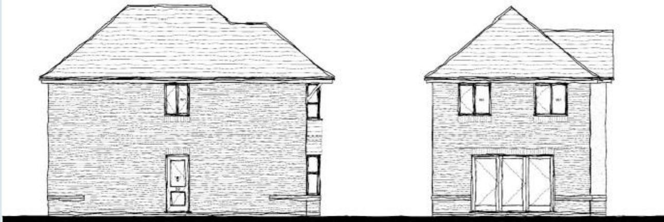
REAR ELEVATION
